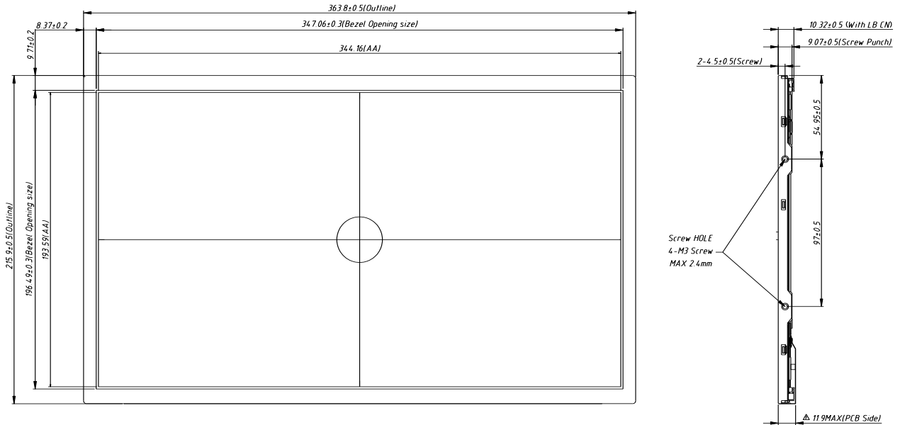
Figure 13 Reference Outline Drawing (Front Side)
