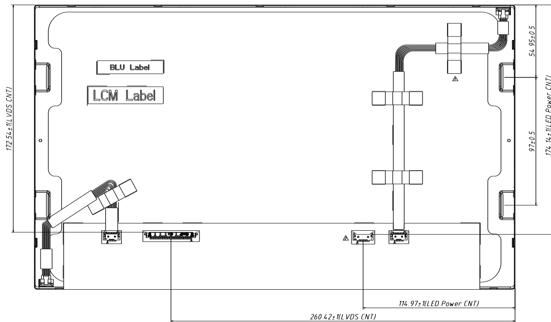
Figure 14 Reference Outline Drawing (Back Side)
