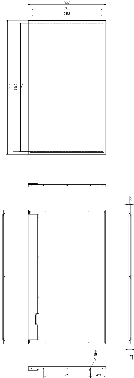
Figure 5. TFT-LCD Module Outline Dimensions (Front view)
