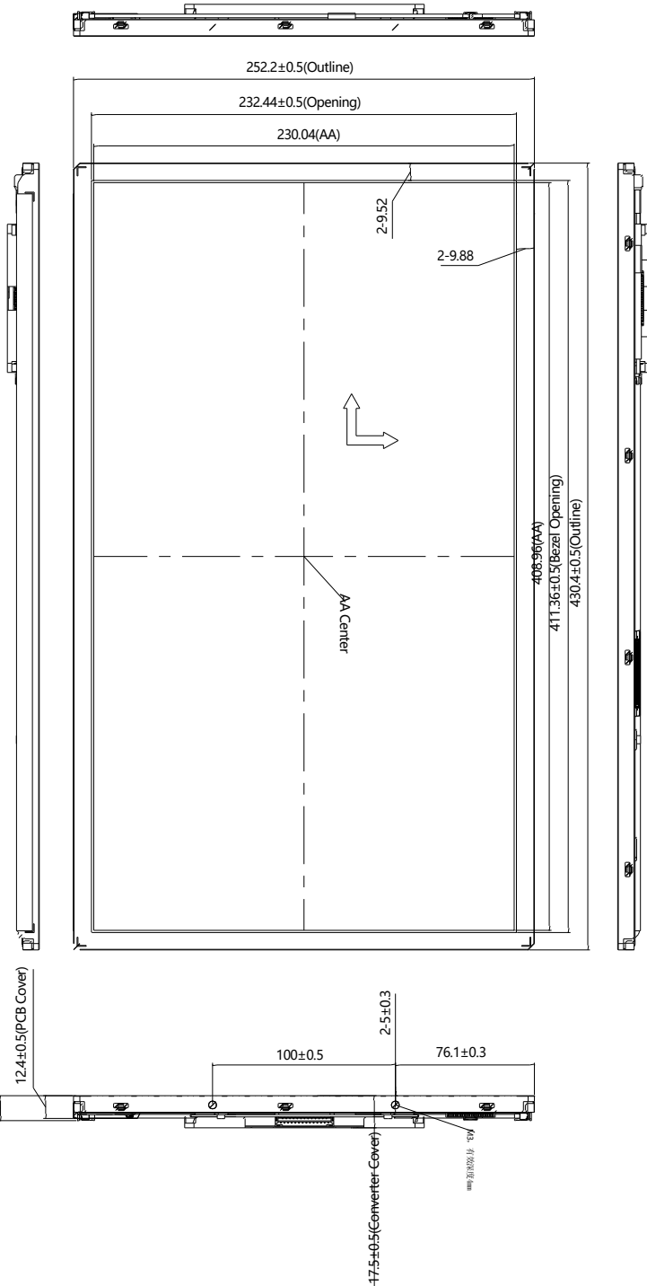
< Figure 3.TFT-LCD Module Outline Dimensions (Front View) >
