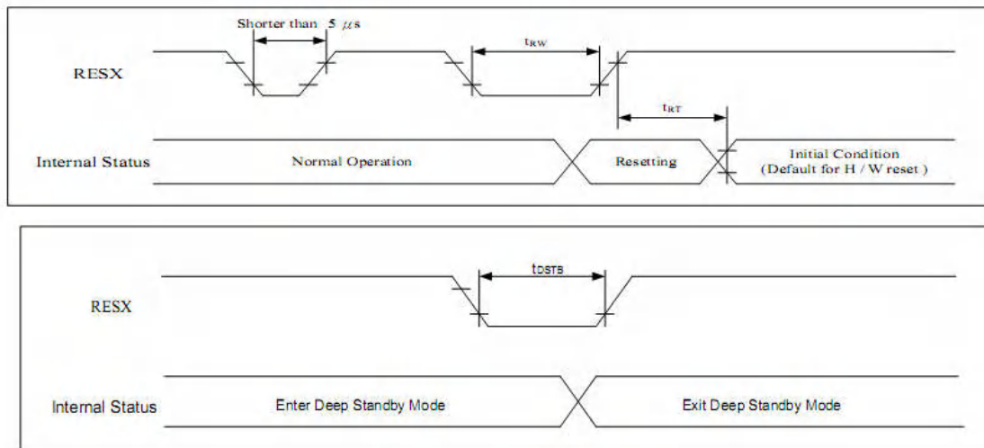
Figure 7.3.4 Reset Operation
