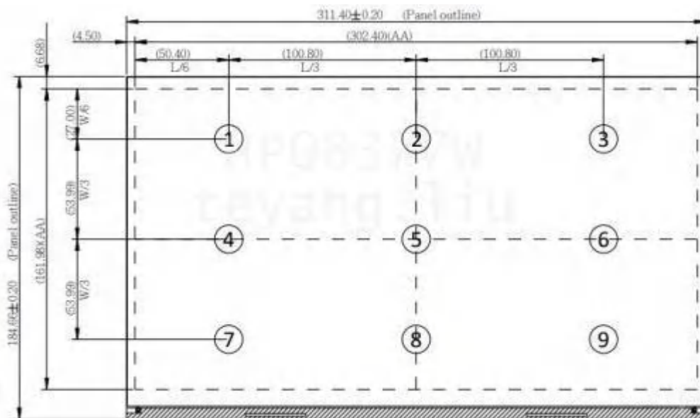
Fig. 2 Definition of luminance uniformity
